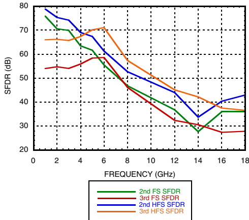
Hold-Mode SFDR vs. Frequency & Input Power @ f_{clk} = 2 \text{ GHz @ 0 dBm}
