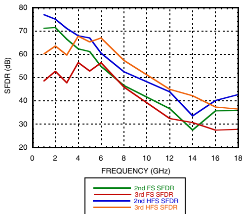
Hold-Mode SFDR vs. Frequency & Input Power @ f_{clk} = 3 \text{ GHz @ 0 dBm}
