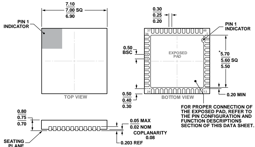
Figure 76. 48-Lead Lead Frame Chip Scale Package [LFCSP_WQ] 7 mm x 7 mm Body, Very Very Thin Quad (CP-48-13) Dimensions shown in millimeters
