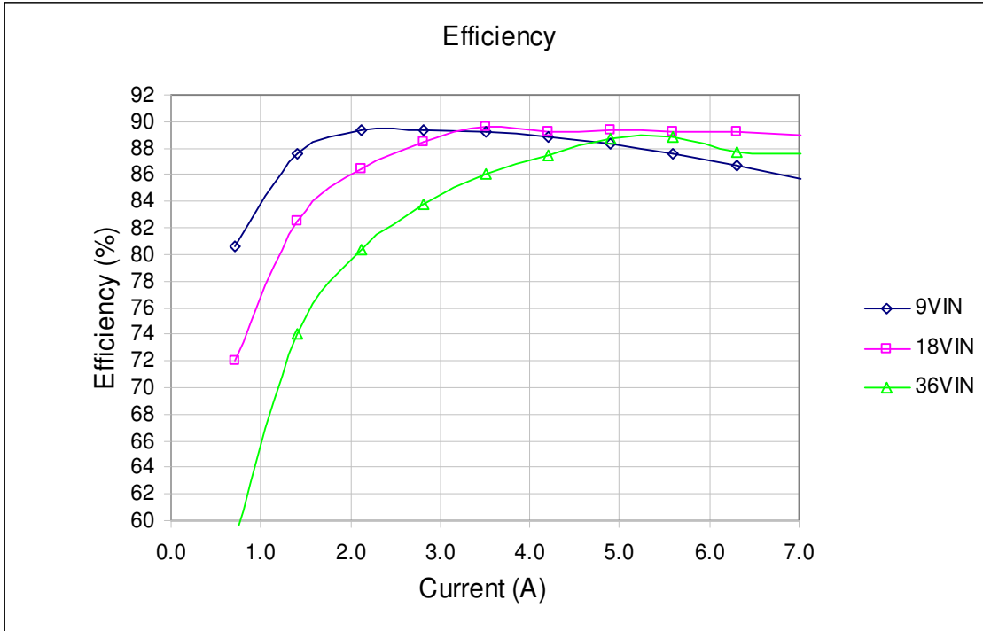
Figure 2. Efficiency
