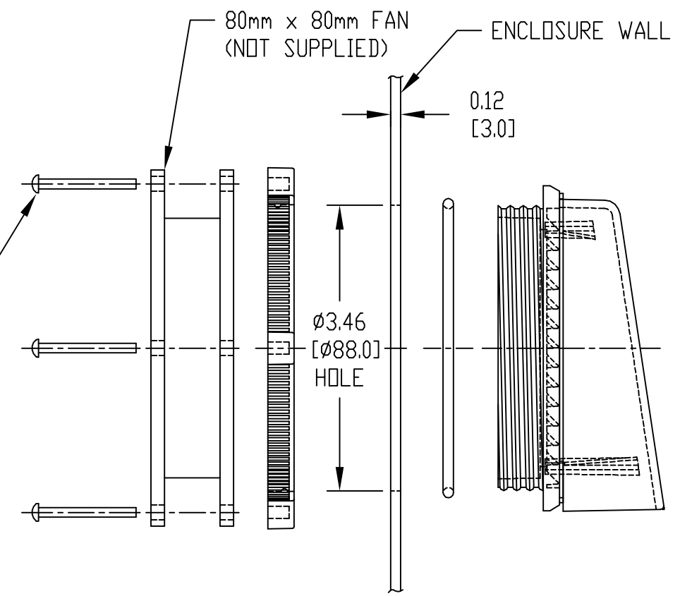
TYPICAL INSTALLATION
