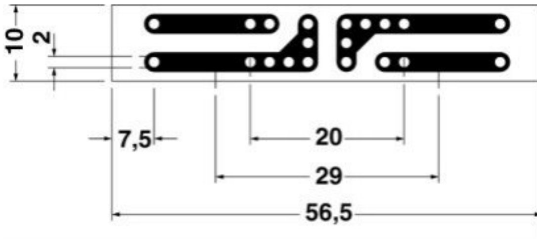
Dimensioned drawing
