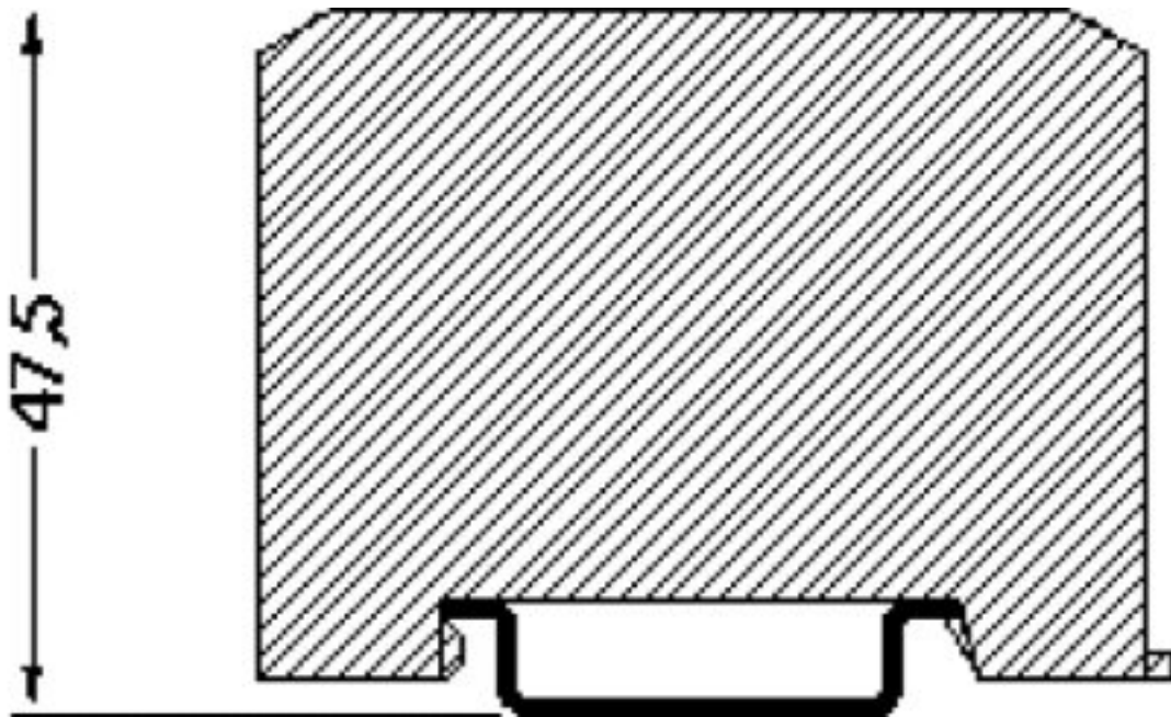
Dimensioned drawing
