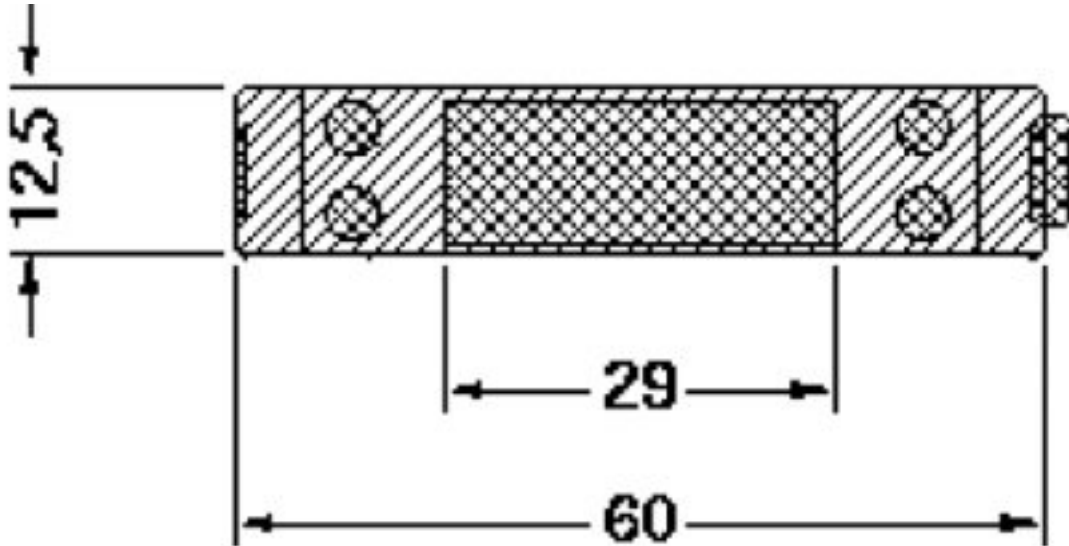
Dimensioned drawing
