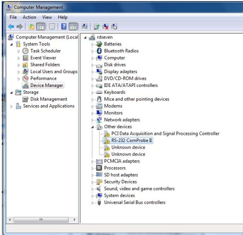
Figure 22 - Device Manager
