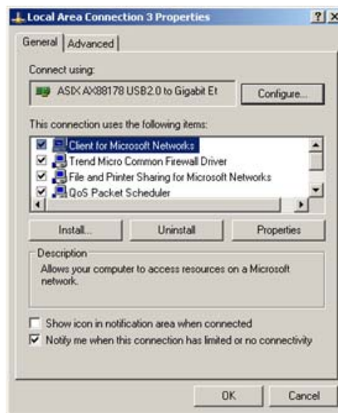
Figure 19 - Properties Dialog
