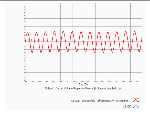
HQA2W085W150V Typical Output Ripple at nominal Input voltage and full load at Ta=25 degree
