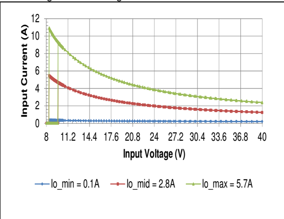
HQA2W085W150V Typical Input Current vs. Input Voltage Characteristics
