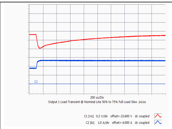
HQA2W085W240V Typical transient response. Output voltage response to load step from 50% to 75% of full load with output current slew rate of 0.1A/uS.
