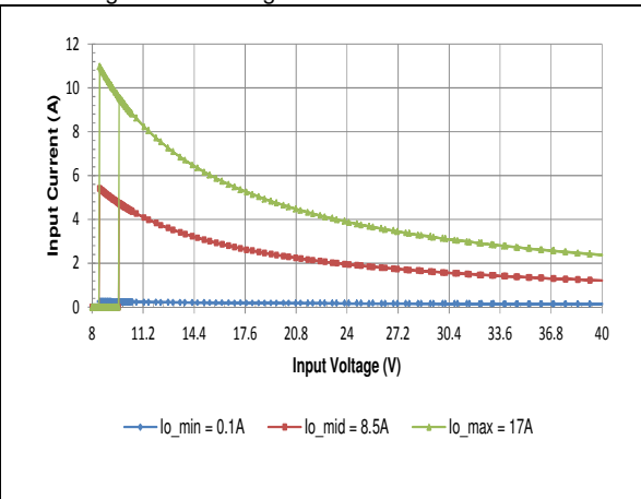
HQA2W085W050V Typical Input Current vs. Input Voltage Characteristics
