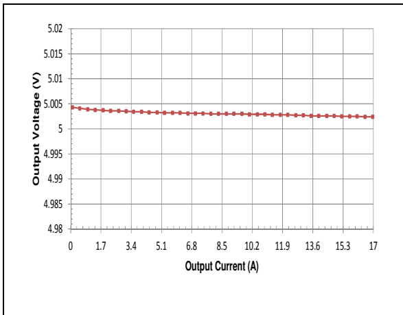
HQA2W085W050V Typical Load Regulation Characteristics at Ta=25 degrees.
