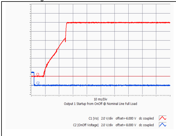
HQA2W085W120V Typical startup characteristic from on/off at full load. Lower trace - on/off signal, upper trace – output voltage
