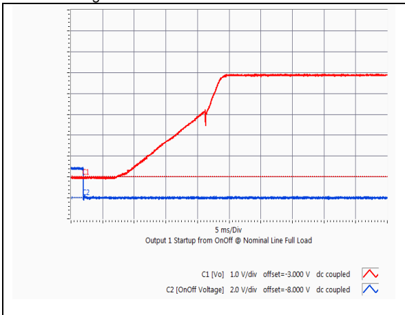
HQA2W085W050V Typical startup characteristic from on/off at full load. Lower trace - on/off signal, upper trace – output voltage
