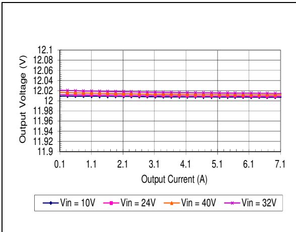
HQA2W085W120V Typical Load Regulation Characteristics at Ta=25 degrees.
