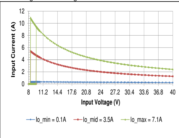
HQA2W085W120V Typical Input Current vs. Input Voltage Characteristics
