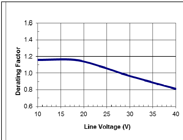
HQA2W085W120V typical temperature derating versus input voltage output with 2m/s (400 lfm) airflow from pin 3 to pin 1.
