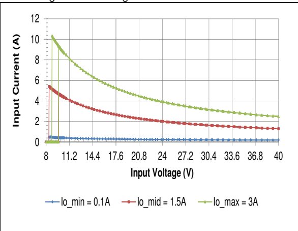
HQA2W085W280V Typical Input Current vs. Input Voltage Characteristics
