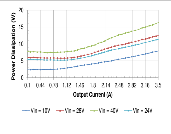
HQA2W085W240V Typical Power Dissipation vs. Input Voltage at Ta=25 degrees
