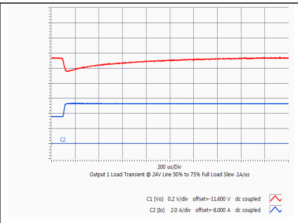
HQA2W085W280V Typical transient response. Output voltage response to load step from 50% to 75% of full load with output current slew rate of 0.1A/uS.
