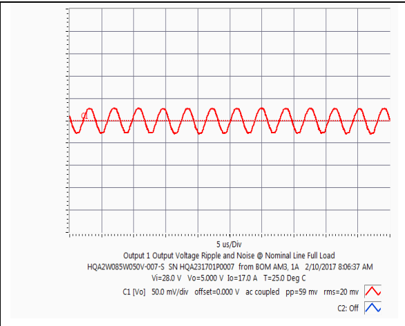
HQA2W085W050V Typical Output Ripple at nominal Input voltage and full load at Ta=25 degree
