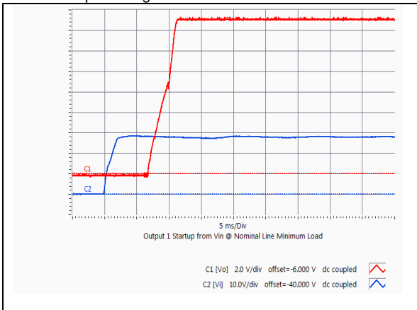
HQA2W085W150V Typical startup characteristic from input voltage application at light load. Red trace - output voltage, Blue trace -input voltage
