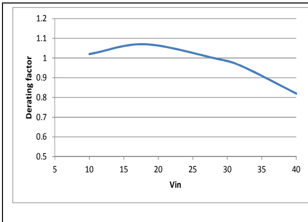
HQA2W085W050V typical temperature derating versus input voltage output with 2m/s (400 lfm) airflow from pin 3 to pin 1.
