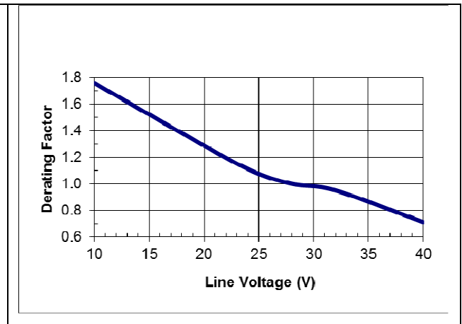
HQA2W085W240V typical temperature derating versus input voltage output with 2m/s (400 lfm) airflow from pin 3 to pin 1.
