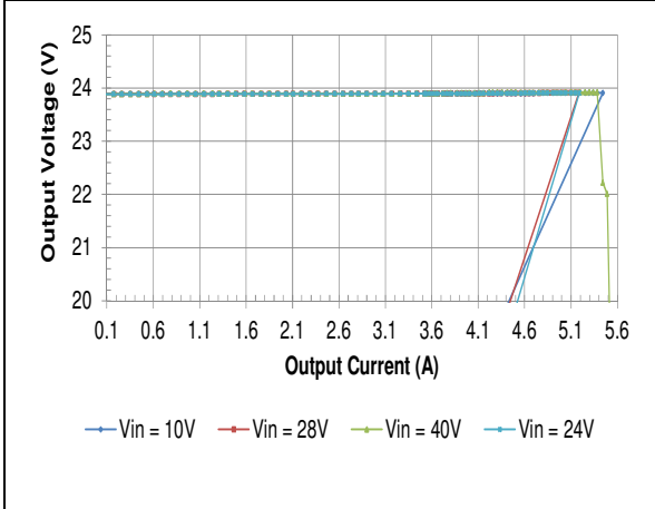
HQA2W085W240V Typical Output Current Limit Characteristics vs. Input Voltage at Ta=25 degrees.
