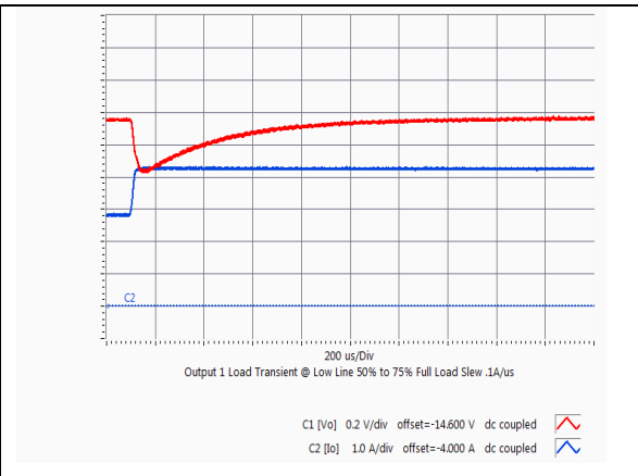
HQA2W085W150V Typical output voltage response to load step from 50% to 75% of full load with output current slew rate of 0.1A/uS and Cext = 10uF
