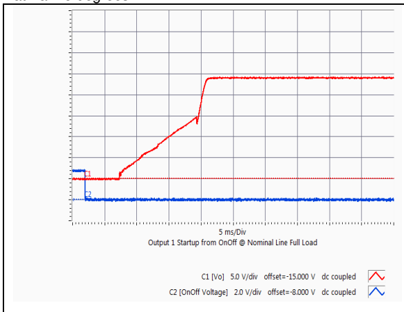
HQA2W085W240V Typical startup characteristic from on/off at full load. Blue trace - on/off signal, red trace – output voltage
