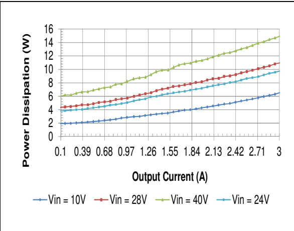
HQA2W085W280V Typical Power Dissipation vs. Input Voltage at Ta=25 degrees
