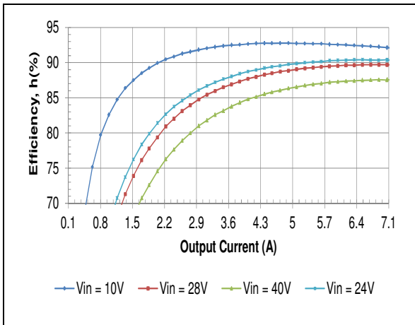
HQA2W085W120V Typical Efficiency vs. Input Voltage at Ta=25 degrees.
