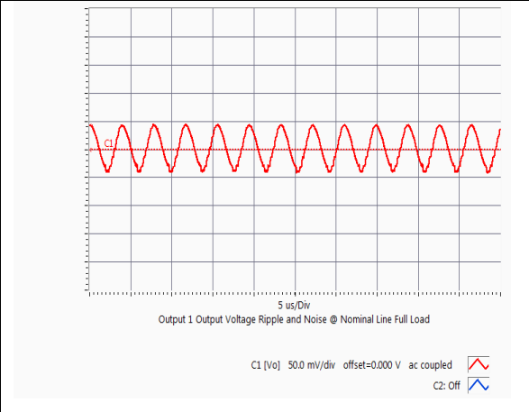
HQA2W085W240V Typical Output Ripple at nominal Input voltage and full load at Ta=25 degree
