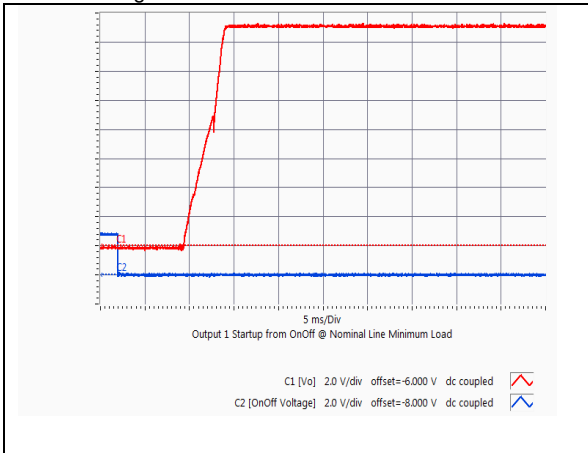
HQA2W085W150V Typical startup characteristic from on/off at light load. Lower trace - on/off signal, upper trace - output voltage
