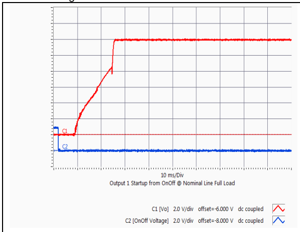
HQA2W085W280V Typical startup characteristic from on/off at full load. Blue trace - on/off signal, red trace – output voltage
