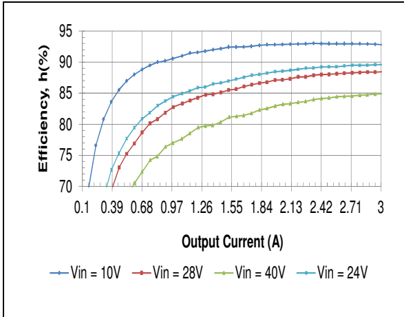
HQA2W085W280V Typical Efficiency vs. Input Voltage at Ta=25 degrees.
