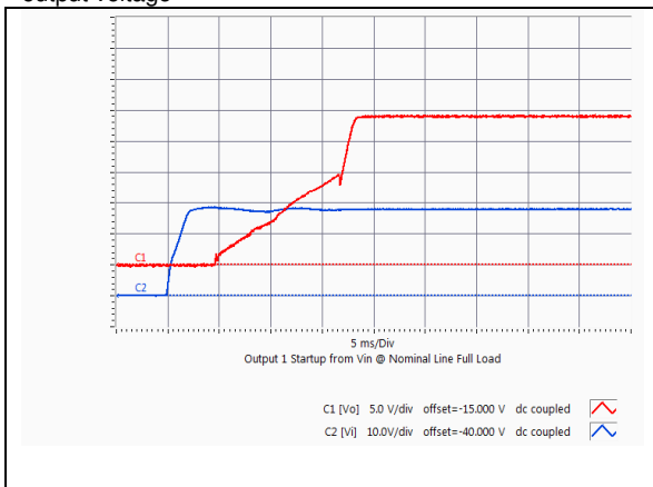
HQA2W085W240V Typical startup characteristic from input voltage application at full load. Red trace - output voltage, blue trace –input voltage
