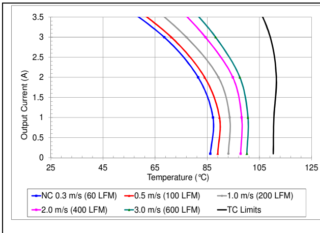
HQA2W085W240V maximum output current vs. ambient temperature at 28V input for airflow rates natural convection (60lfm) to 600lfm with airflow from pin 3 to pin 1
