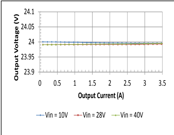
HQA2W085W240V Typical Load Regulation Characteristics at Ta=25 degrees.
