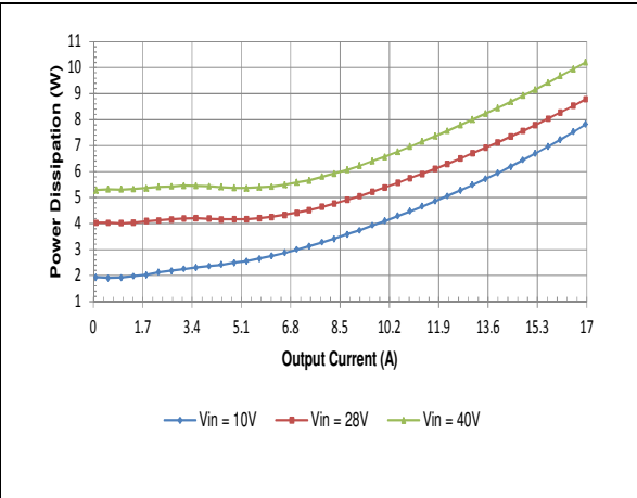
HQA2W085W050V Typical Power Dissipation vs. Input Voltage at Ta=25 degrees
