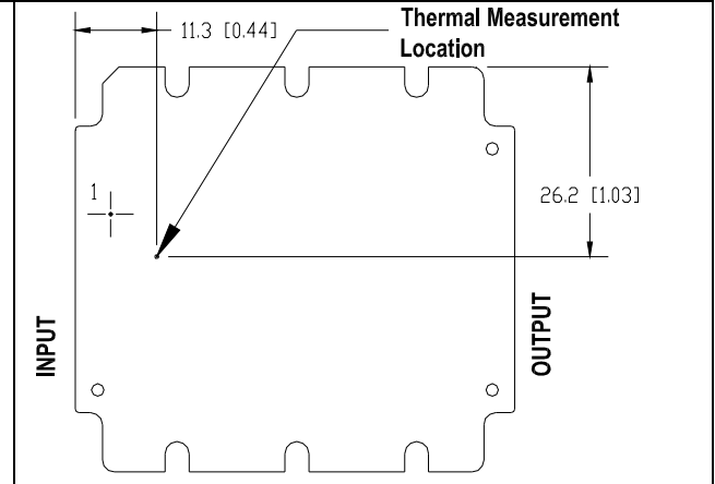
HQA2W085W120V thermal measurement location – top view
