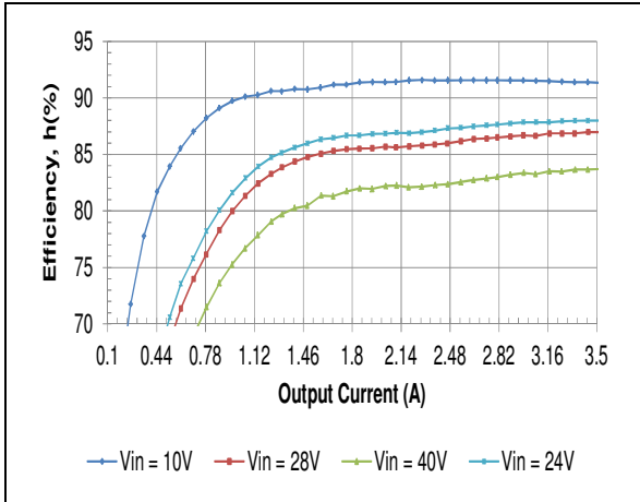
HQA2W085W240V Typical Efficiency vs. Input Voltage at Ta=25 degrees.
