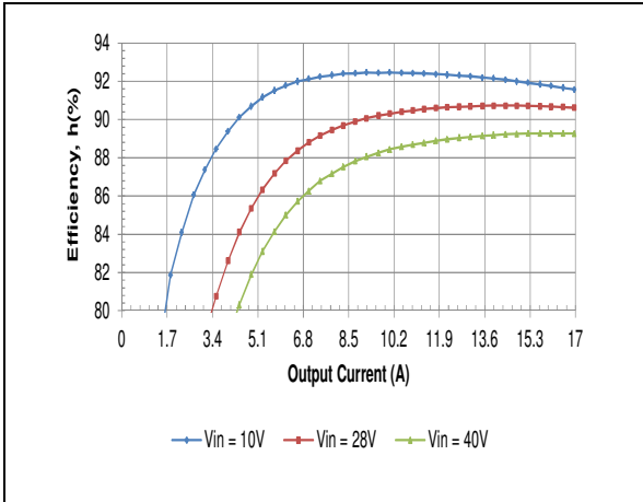
HQA2W085W050V Typical Efficiency vs. Input Voltage at Ta=25 degrees.
