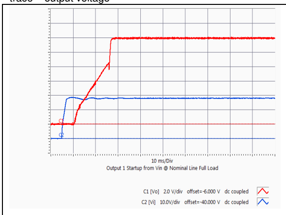
HQA2W085W120V Typical startup characteristic from input voltage application at full load. Red trace - output voltage, Blue trace –input voltage
