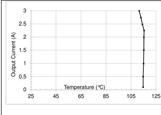
HQA2W085W280V maximum output current vs. baseplate temperature
