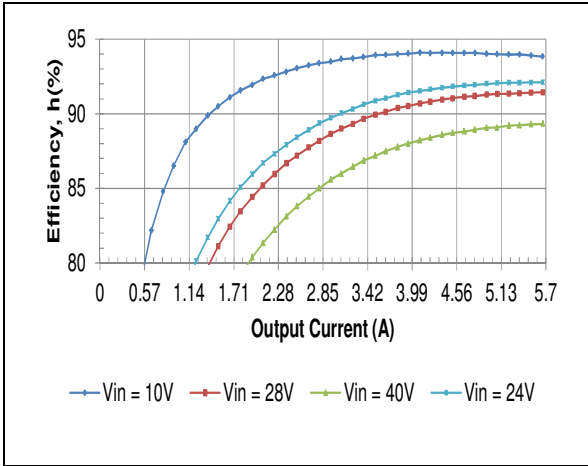
HQA2W085W150V Typical Efficiency vs. Input Voltage at Ta=25 degrees.
