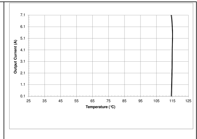
HQA2W085W120V maximum output current vs. baseplate temperature at nominal line
