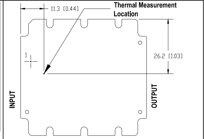
HQA2W085W050V thermal measurement location – top view
