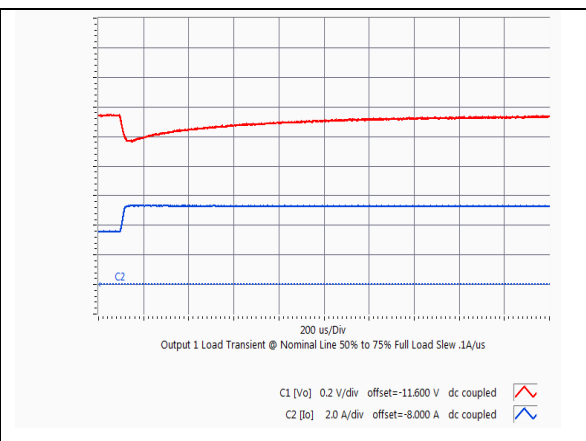
HQA2W085W120V Typical output voltage response to load step from 50% to 75% of full load with output current slew rate of 0.1A/μs and Cext = 500μF
