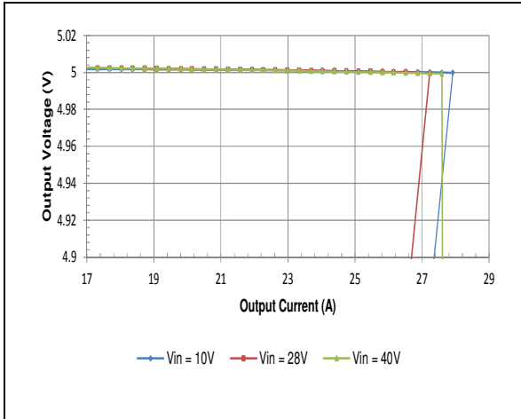
HQA2W085W050V Typical Output Current Limit Characteristics vs. Input Voltage at Ta=25 degrees.
