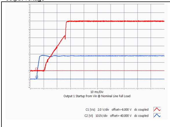
HQA2W085W280V Typical startup characteristic from input voltage application at full load. Red trace - output voltage, blue trace –input voltage
