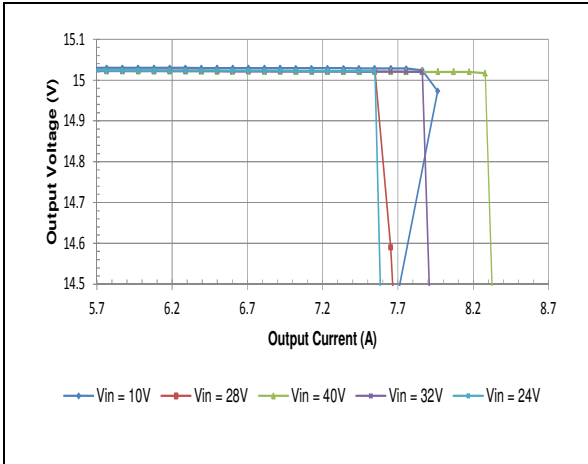
HQA2W085W150V Typical Output Current Limit Characteristics vs. Input Voltage at Ta=25 degrees.
