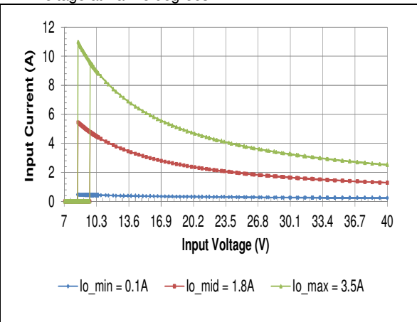
HQA2W085W240V Typical Input Current vs. Input Voltage Characteristics
