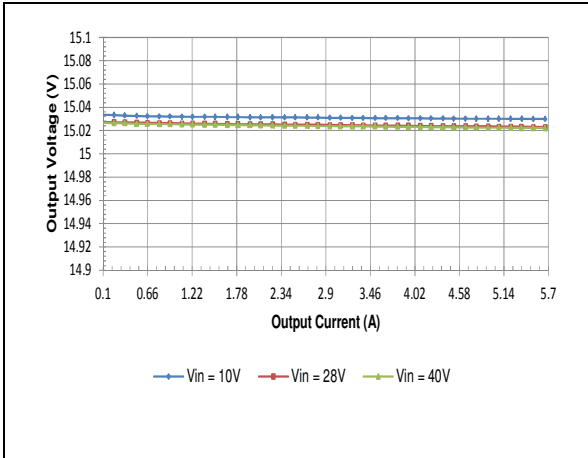
HQA2W085W150V Typical Load Regulation Characteristics at Ta=25 degrees.
