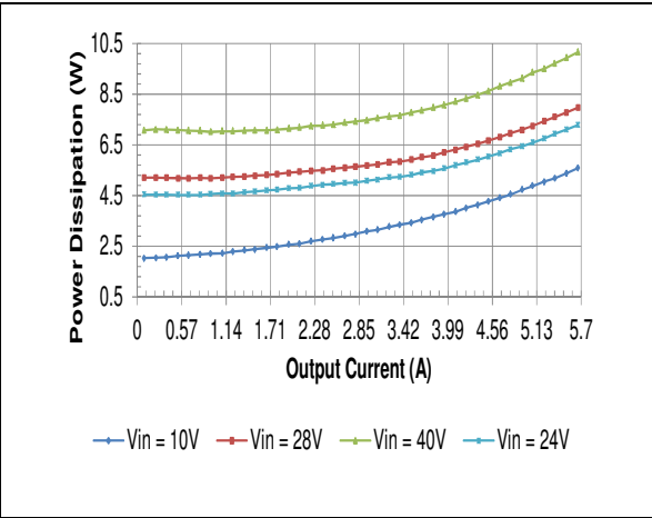
HQA2W085W150V Typical Power Dissipation vs. Input Voltage at Ta=25 degrees
