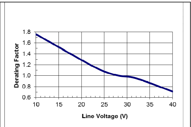
HQA2W085W280V typical temperature derating versus input voltage output with 2m/s (400 lfm) airflow from pin 3 to pin 1.
