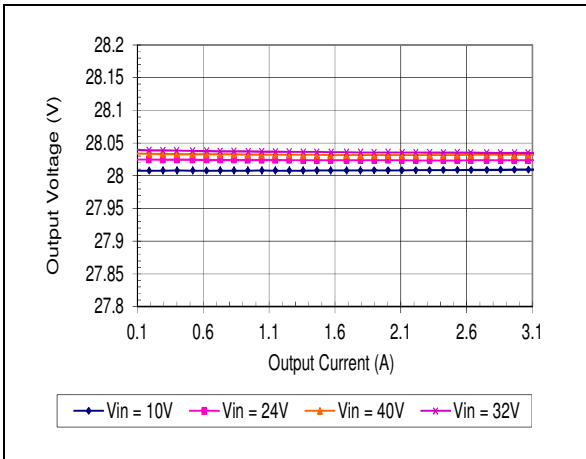
HQA2W085W280V Typical Load Regulation Characteristics at Ta=25 degrees.
