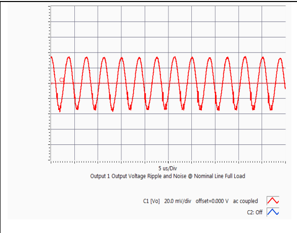
HQA2W085W120V Typical Output Ripple at nominal Input voltage and full load at Ta=25 degree
