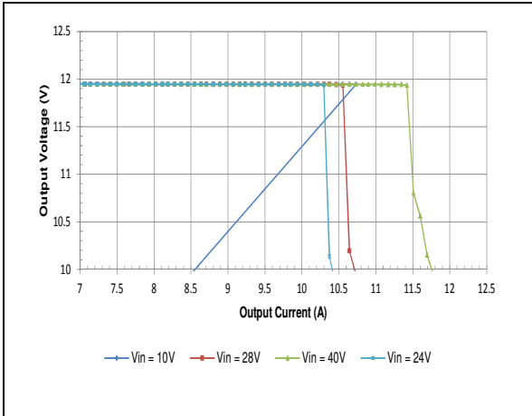
HQA2W085W120V Typical Output Current Limit Characteristics vs. Input Voltage at Ta=25 degrees.
