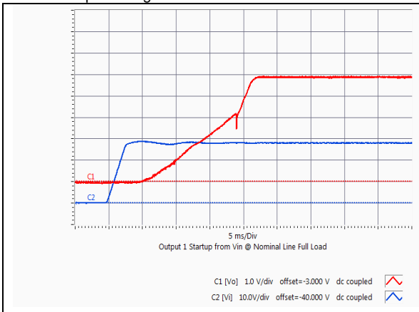
HQA2W085W050V Typical startup characteristic from input voltage application at full load. Red trace - output voltage, Blue trace –input voltage
