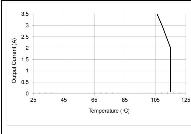
HQA2W085W240V maximum output current vs. baseplate temperature at nominal line
