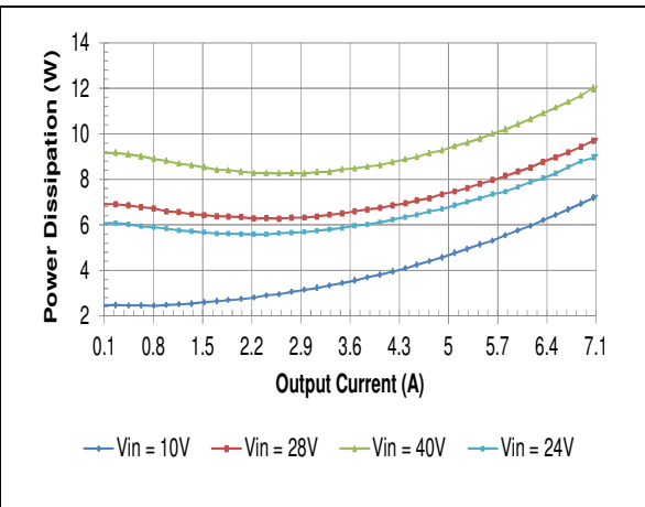
HQA2W085W120V Typical Power Dissipation vs. Input Voltage at Ta=25 degrees
