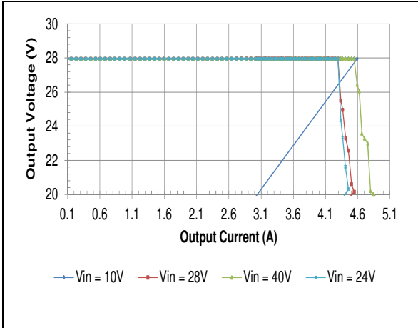
HQA2W085W280V Typical Output Current Limit Characteristics vs. Input Voltage at Ta=25 degrees.
