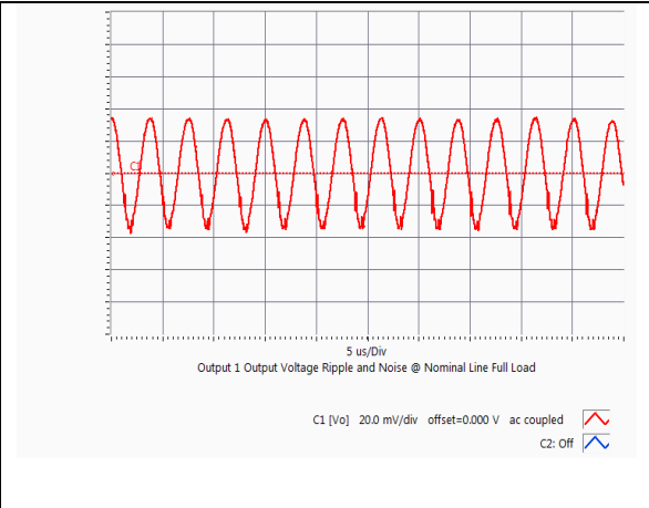
HQA2W085W280V Typical Output Ripple at nominal Input voltage and full load at Ta=25 degree
